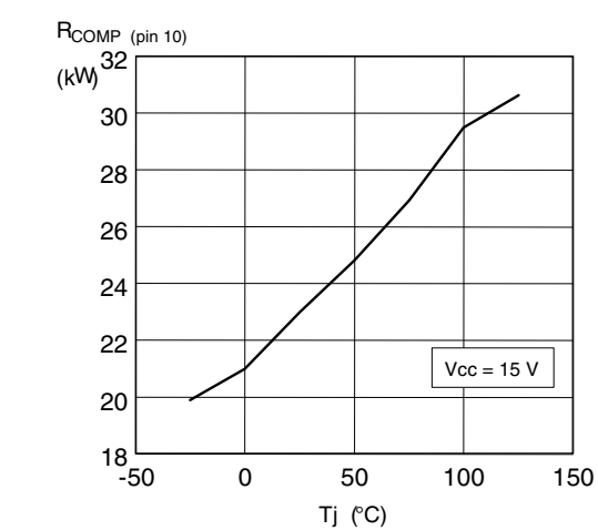
Figure 15. COMP dynamic resistance vs. Tj
