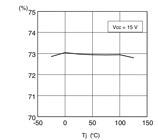
Figure 16. Max. duty-cycle vs. Tj
