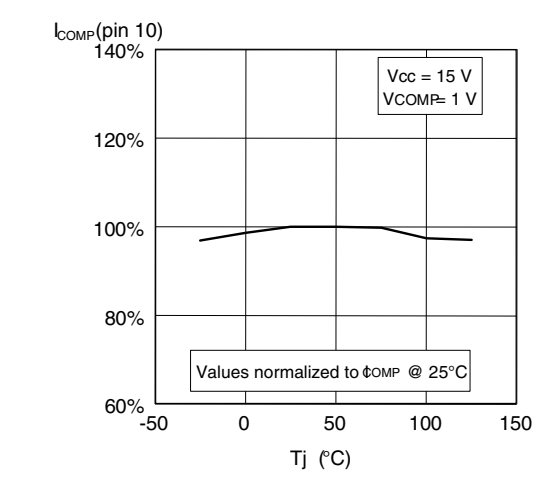
Figure 14. COMP source current vs. Tj
