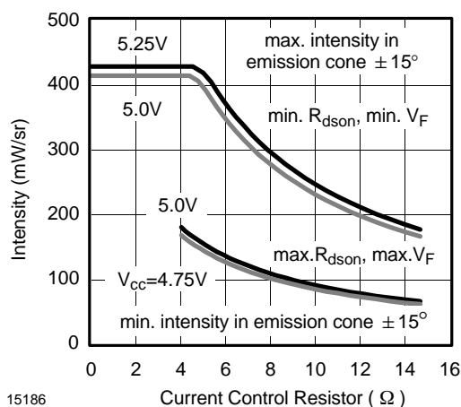
Figure 8. Intensity I_e vs. Current Control Resistor R2 5 V Applications
