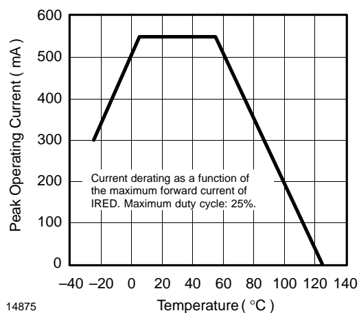
Figure 5. Current Derating Diagram
