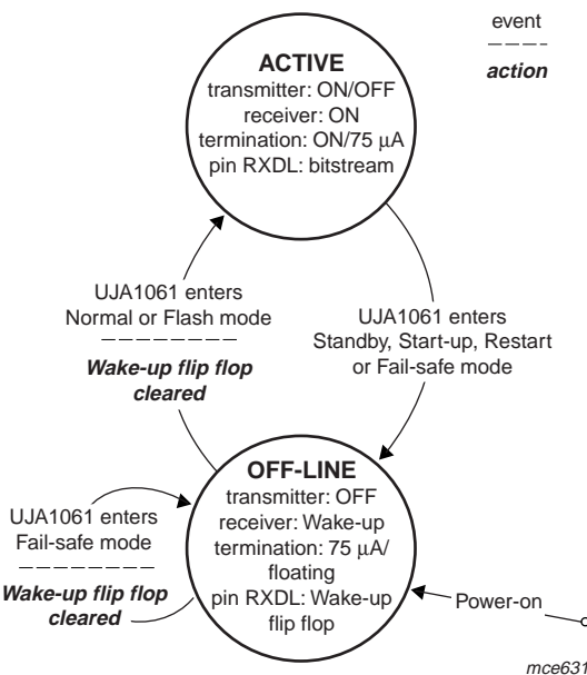
Fig.10 States LIN transceiver.
