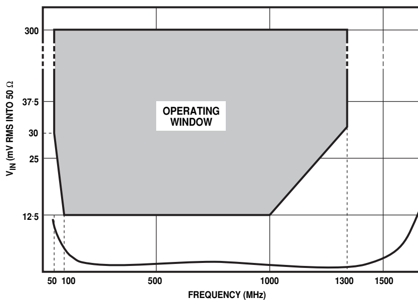
Fig. 5 Typical input sensitivity
