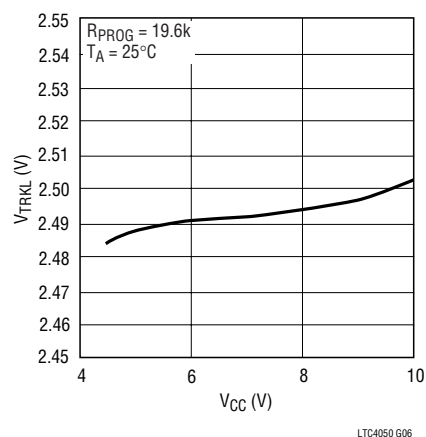
Trickle Charge Threshold Voltage vs V_{CC}
