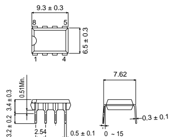
DIP8
