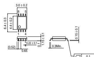
SSOP-B8
