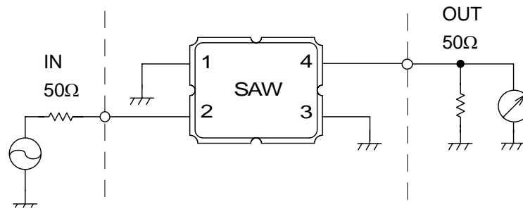
Fig.1 Measuring circuit
