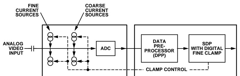
Figure 9. Clamping Overview
