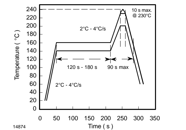
Figure 5. Infrared Reflow Soldering Profile
