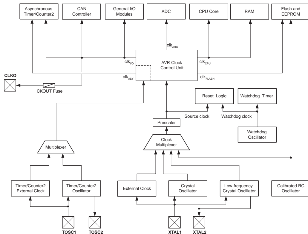
Figure 19. Clock Distribution
