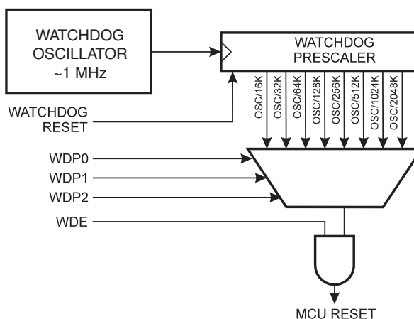
Figure 29. Watchdog Timer
