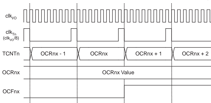
Figure 58. Timer/Counter Timing Diagram, Setting of OCFnx, with Prescaler ( f_{clk\_I/O}/8 )
