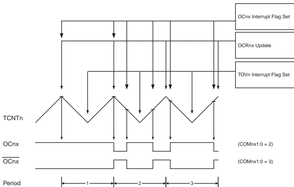
Figure 68. Phase Correct PWM Mode, Timing Diagram
