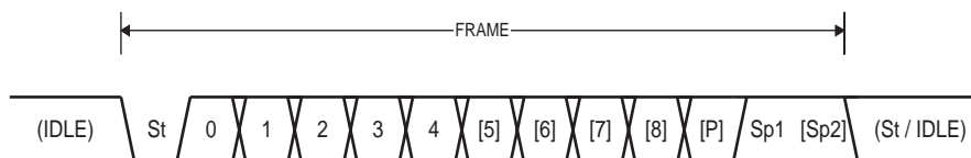
Figure 86. Frame Formats
