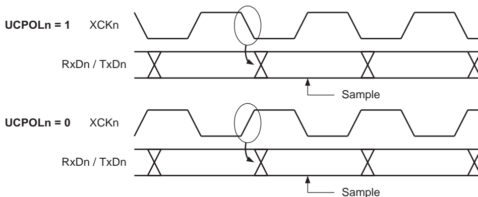
Figure 85. Synchronous Mode XCKn Timing.
