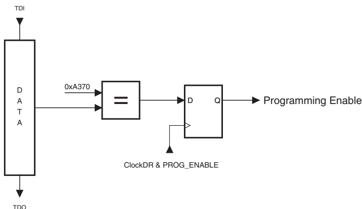
Figure 165. Programming Enable Register
