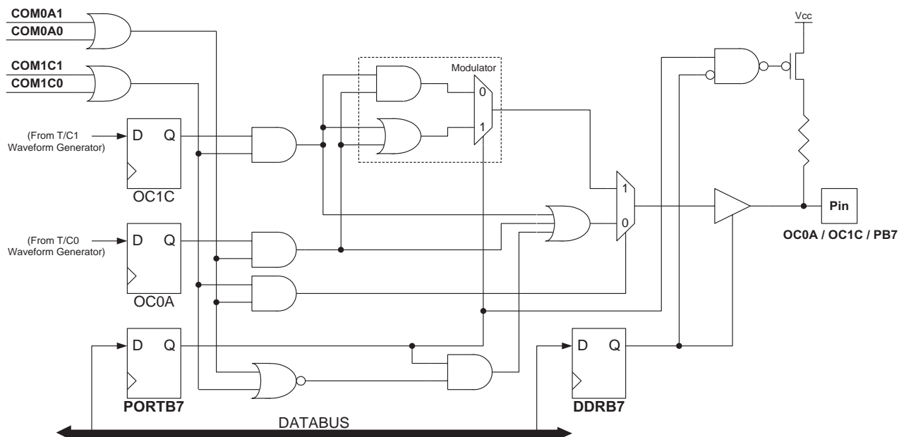
Figure 77. Output Compare Modulator, Schematic
