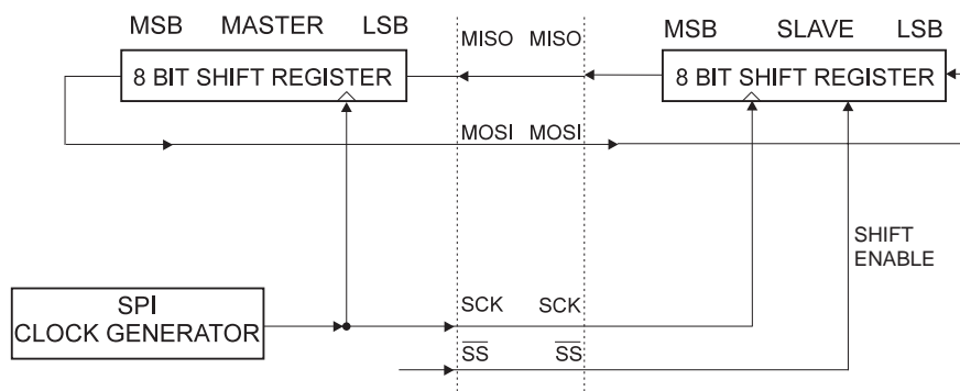
Figure 80. SPI Master-slave Interconnection
