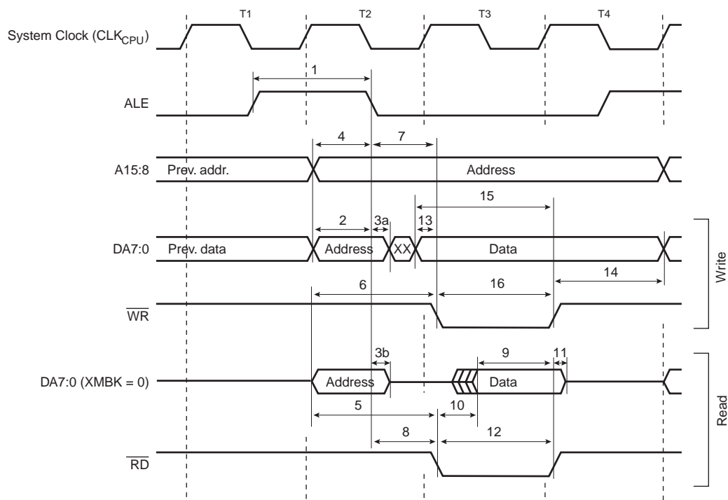
Figure 173. External Memory Timing (SRWn1 = 0, SRWn0 = 0)
