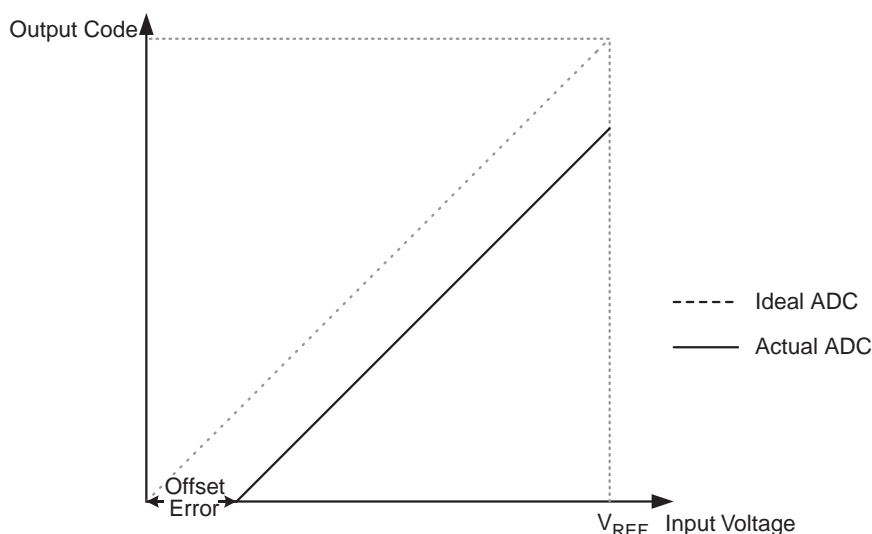
Figure 136. Offset Error
