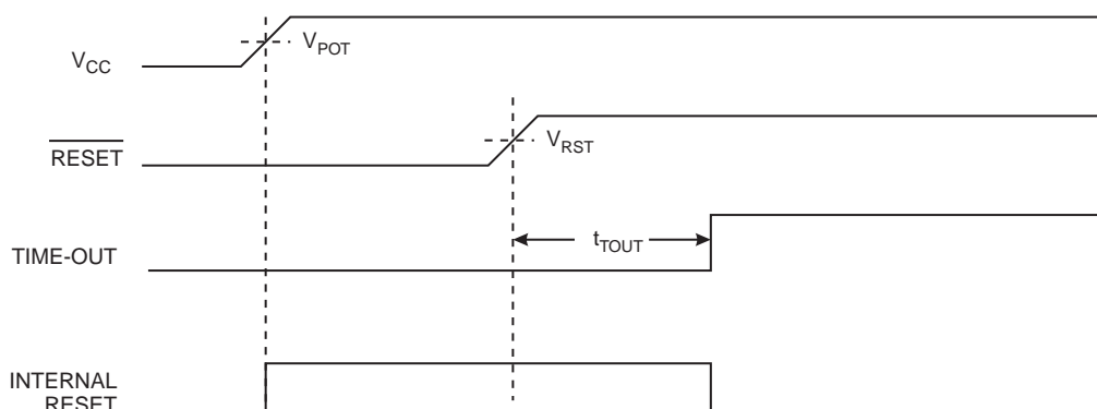
Figure 25. MCU Start-up, \overline{\text{RESET}} Extended Externally
