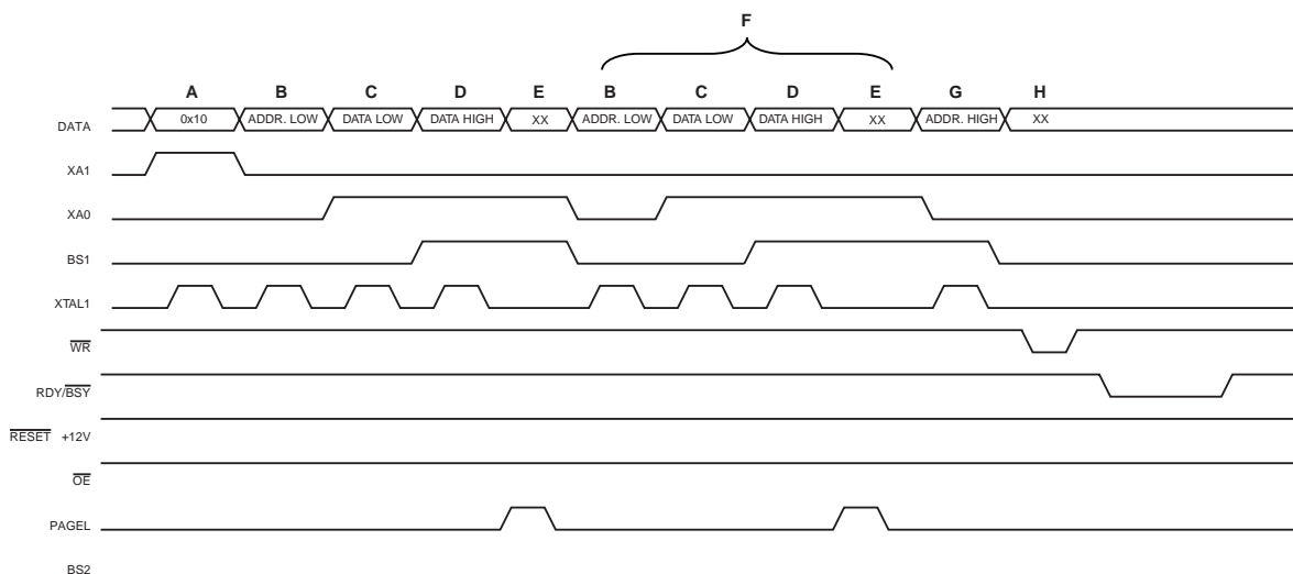
Figure 158. Programming the Flash Waveforms (1)
