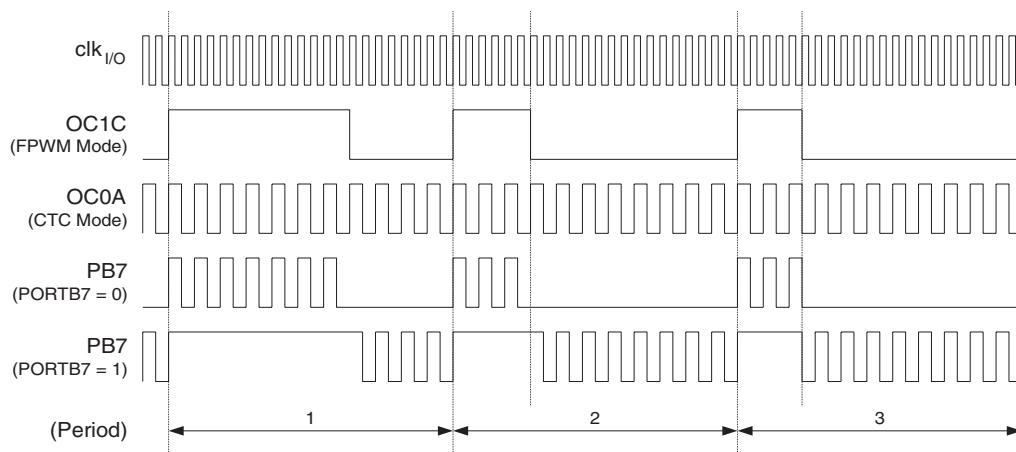
Figure 78. Output Compare Modulator, Timing Diagram
