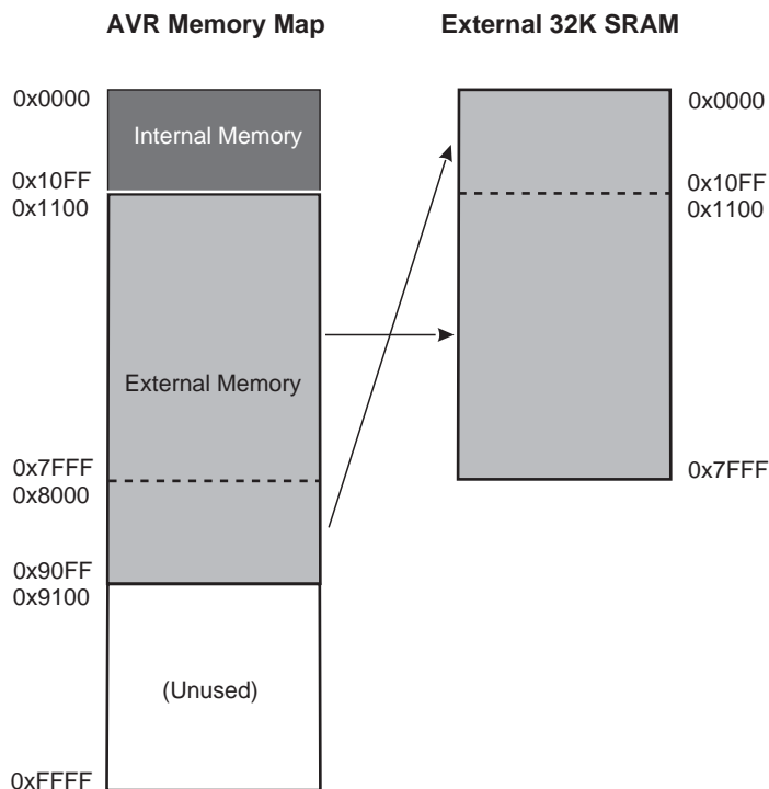
Figure 18. Address Map with 32 KB External Memory
