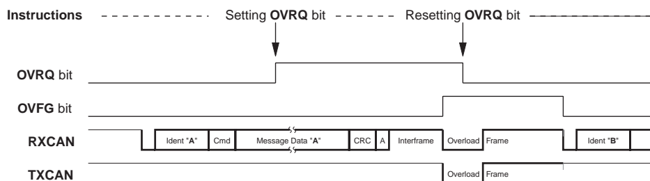
Figure 119. Overload Frame
