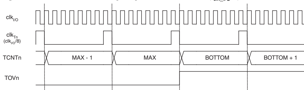
Figure 45. Timer/Counter Timing Diagram, with Prescaler ( f_{clk\_I/O}/8 )
