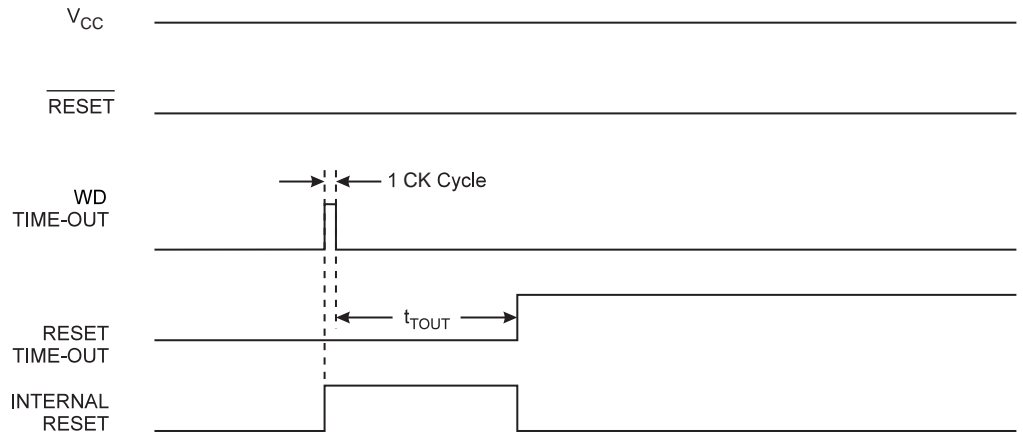
Figure 28. Watchdog Reset During Operation
