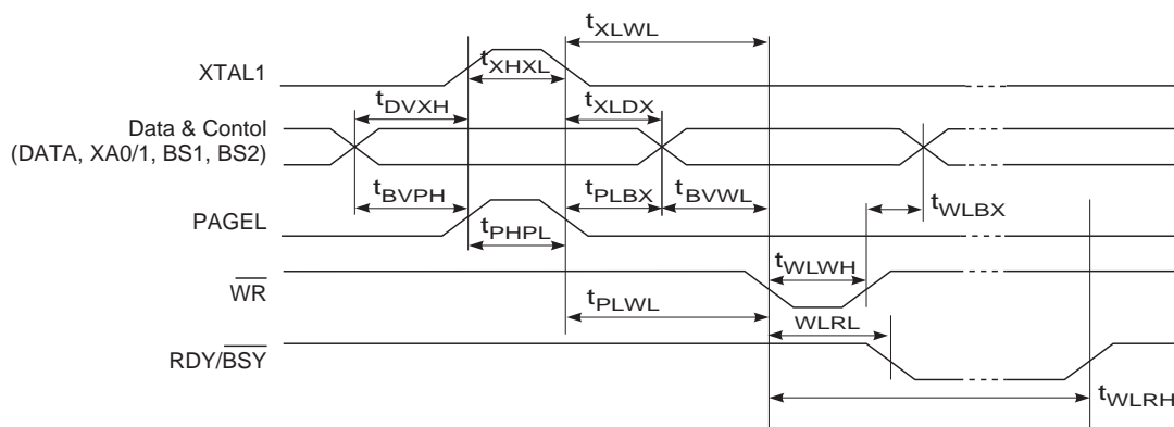
Figure 177. Parallel Programming Timing, Including some General Timing Requirements
