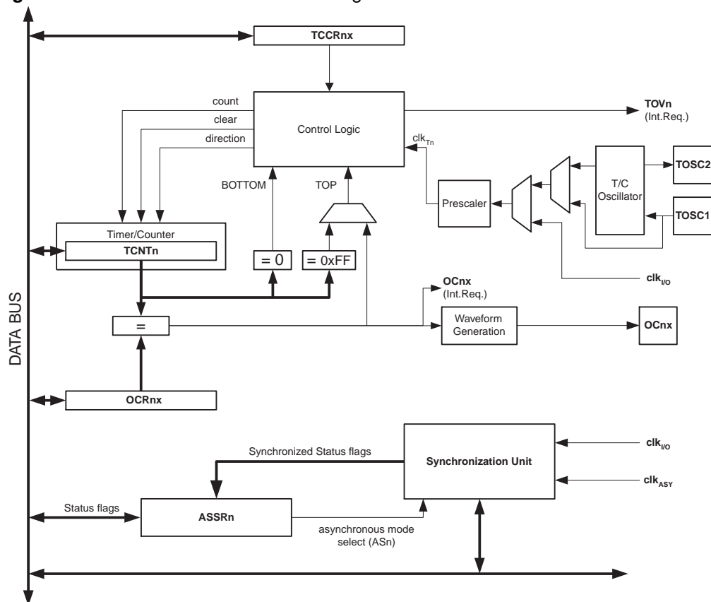
Figure 61. 8-bit Timer/Counter2 Block Diagram
