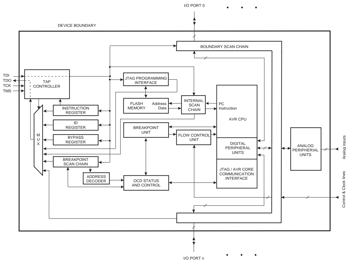
Figure 141. Block Diagram
