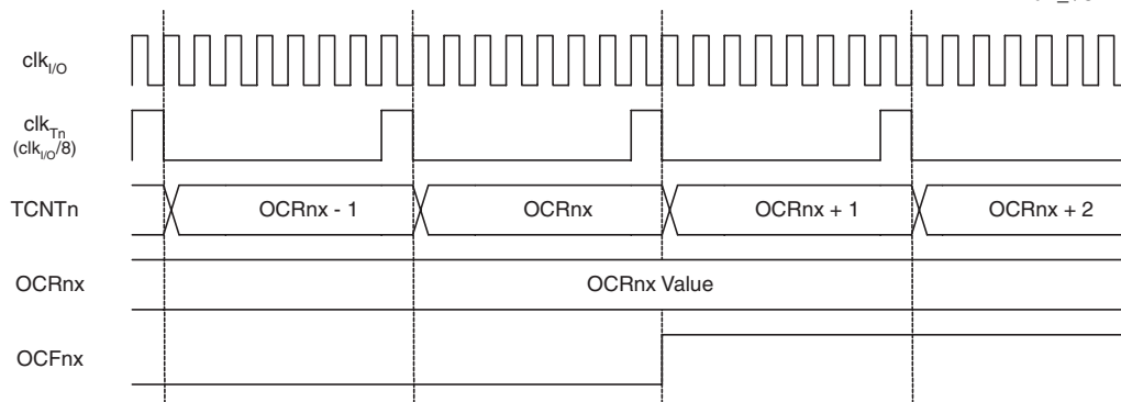
Figure 46. Timer/Counter Timing Diagram, Setting of OCF0A, with Prescaler ( f_{clk\_I/O}/8 )
