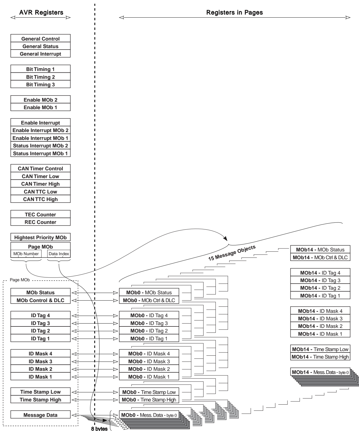
Figure 125. Registers Organization
