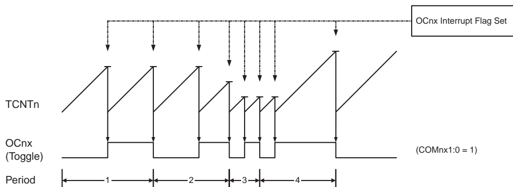
Figure 41. CTC Mode, Timing Diagram
