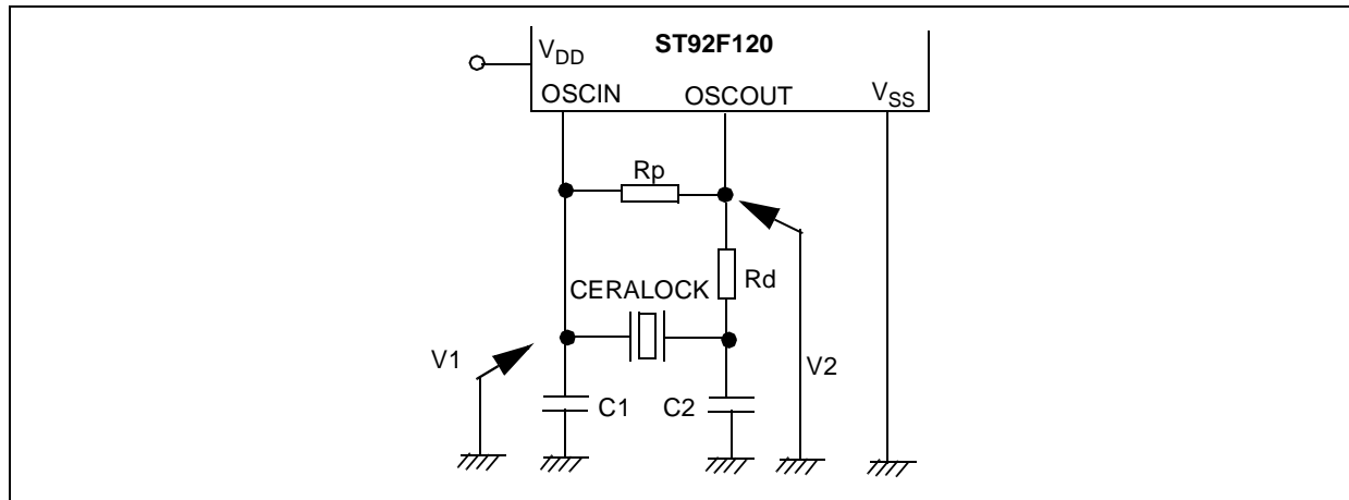
Figure 52. Test Circuit
