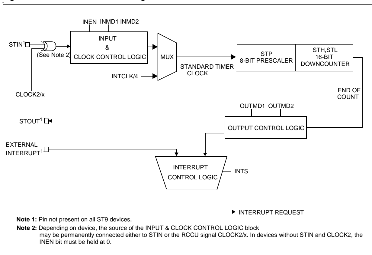
Figure 72. Standard Timer Block Diagram
