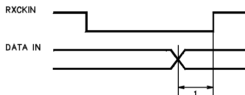
FIG 1: RECEPTION WITH EXTERNAL CLOCK 1X MODE
