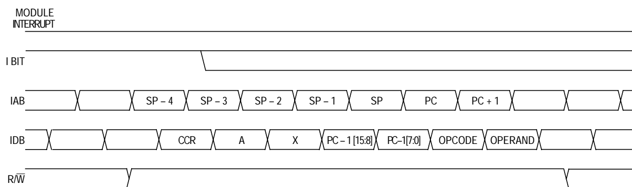
Figure 9-9. Hardware Interrupt Recovery
