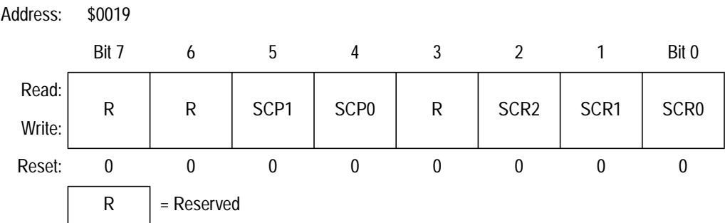
Figure 17-13. SCI BAUD Rate Register 1 (SCBR)
