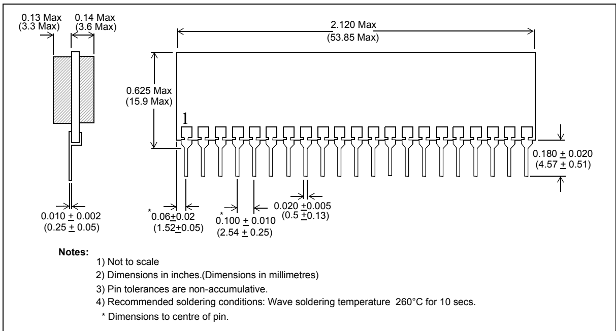
Figure 9 - Mechanical Data
