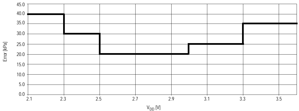
Figure 13. Pressure Error vs V DD at T = 25°C, 500 kPa ≤ P ≤ 900kPa
