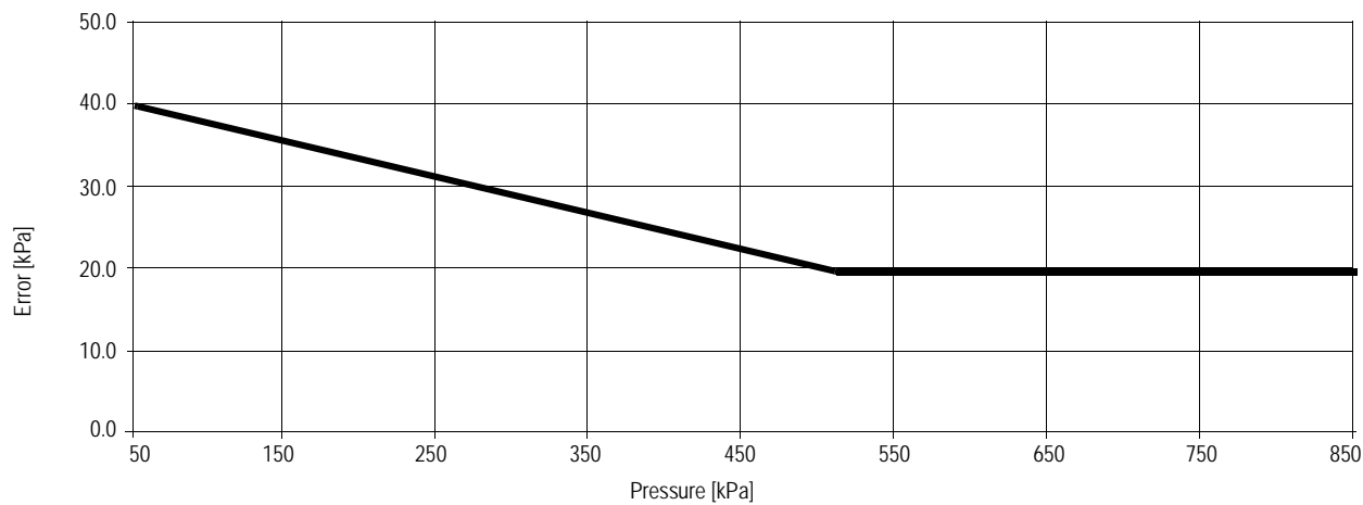
Figure 12. Pressure Error vs Pressure at T= 25°C, 2.5 V ≤ V DD ≤ 3.0 V
