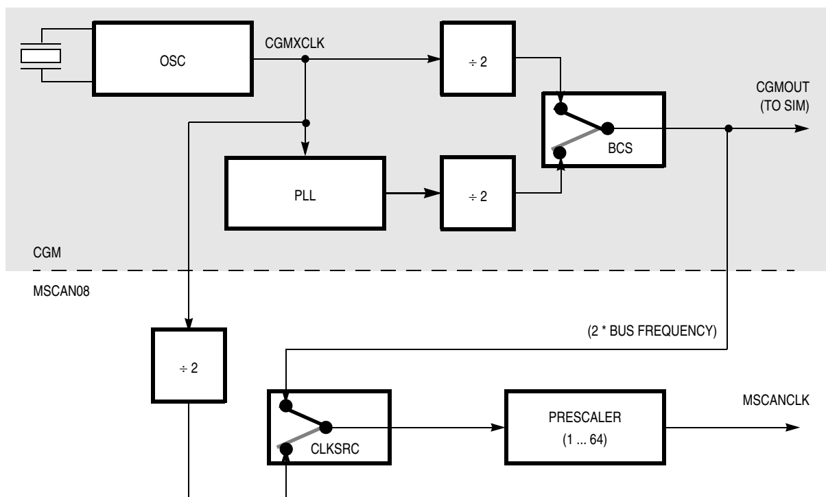
Figure 16-7. Clocking Scheme
