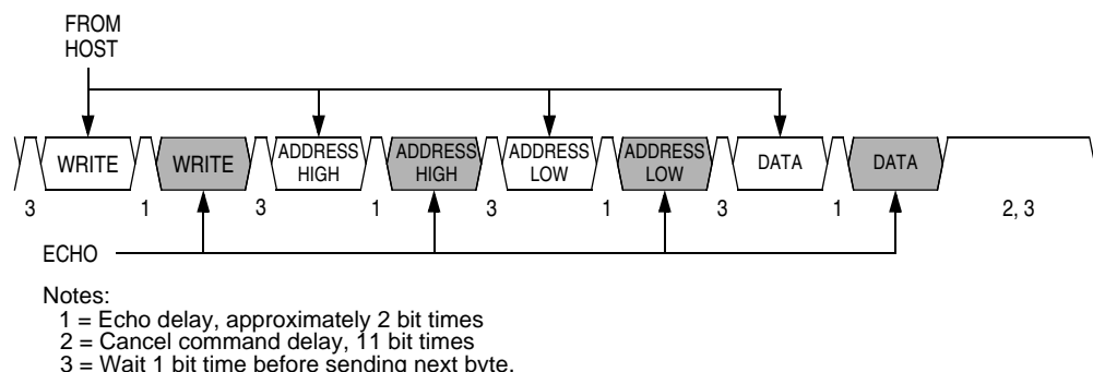
Figure 15-7. Write Transaction
