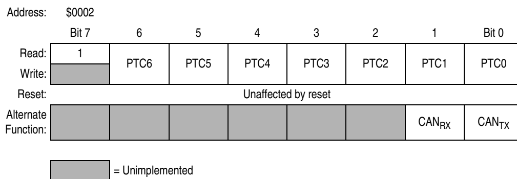
Figure 17-9. Port C Data Register (PTC)
