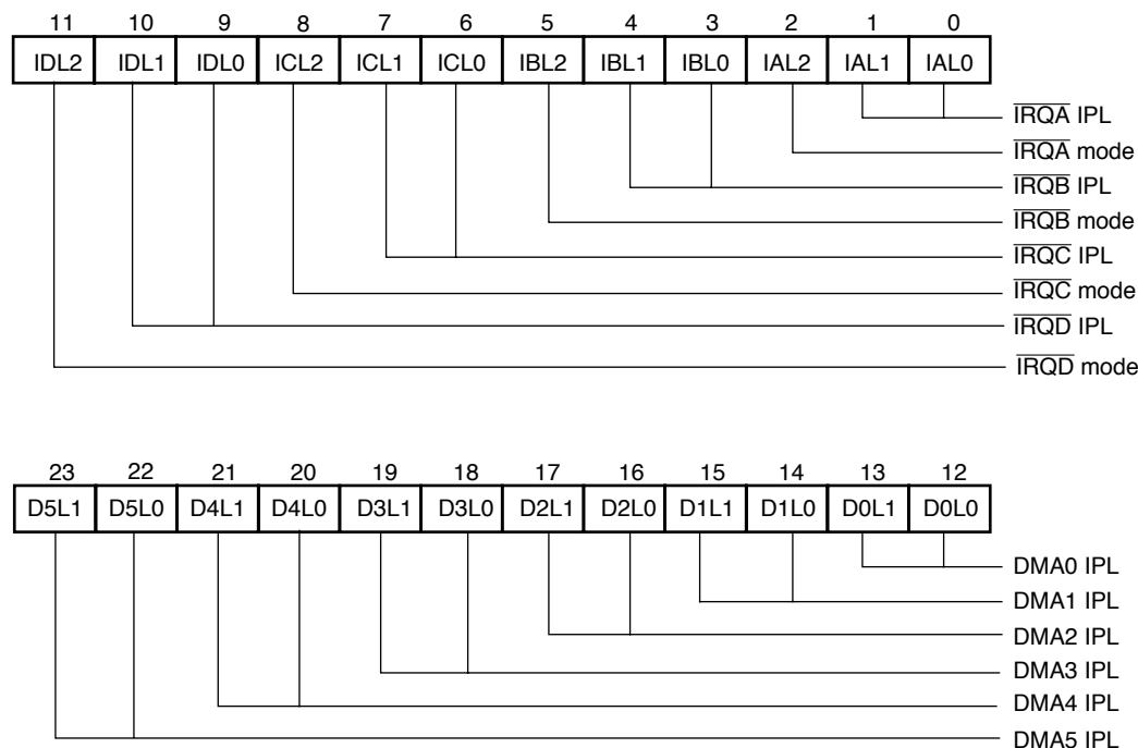
Figure 4-1 Interrupt Priority Register C (IPR-C) (X:$FFFFFF)
