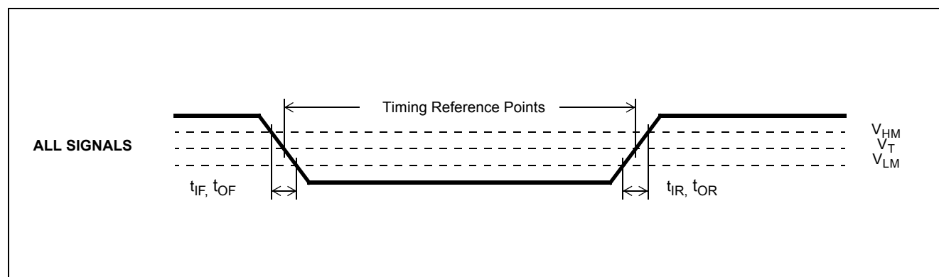
Figure 15 - Timing Parameter Measurement Voltage Levels
