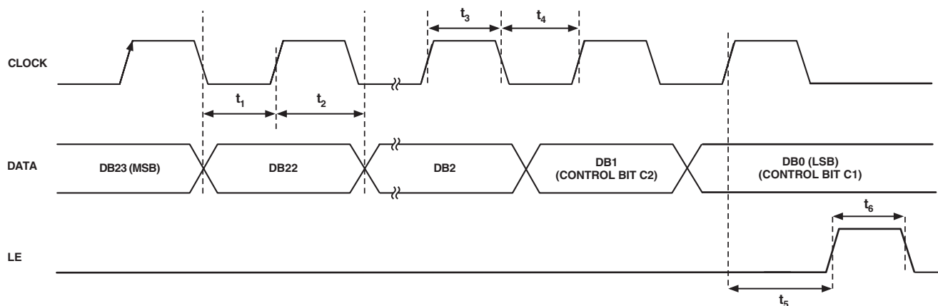
Figure 1. Timing Diagram
