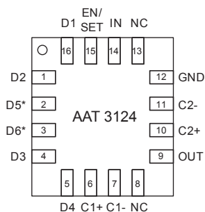
16 LD 4x4mm QFN (Top View)
