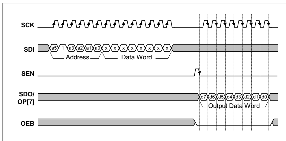
Figure 16 Serial Interface Register Read-back
