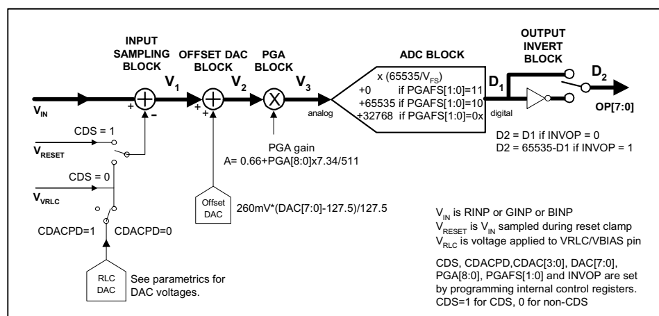
Figure 13 Overall Signal Flow
