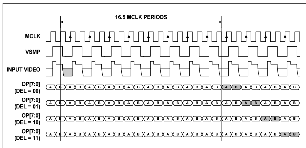
Figure 21 Mode 4 Operation
