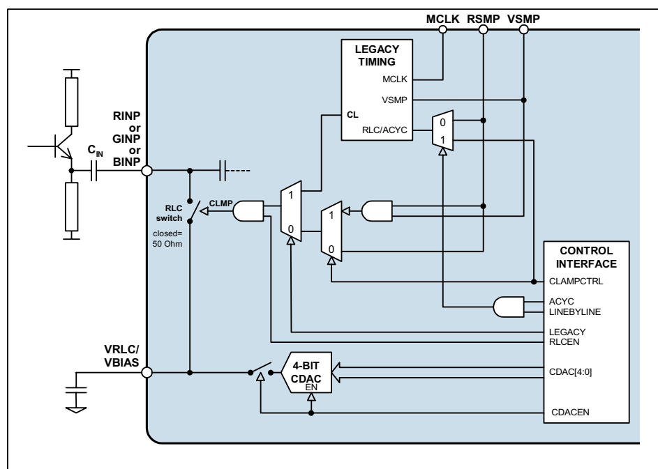
Figure 5 RLC Clamp Control Options
