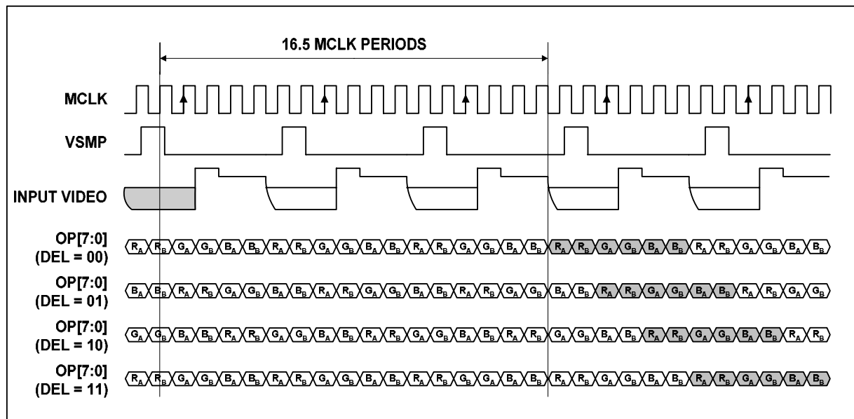
Figure 18 Mode 1 Operation
