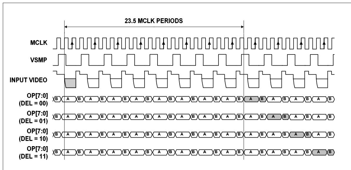
Figure 20 Mode 3 Operation
