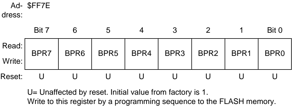
Figure 4-3. FLASH Block Protect Register (FLBPR)
