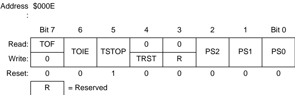
Figure 11-4. TIMA Status and Control Register (TASC)
