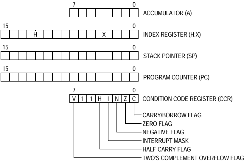
Figure 6-1. CPU Registers
