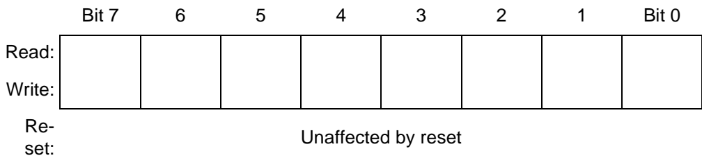
Figure 6-2. Accumulator (A)
