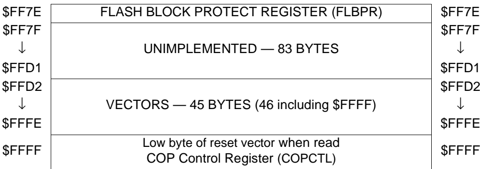
Figure 2-1. Memory Map
