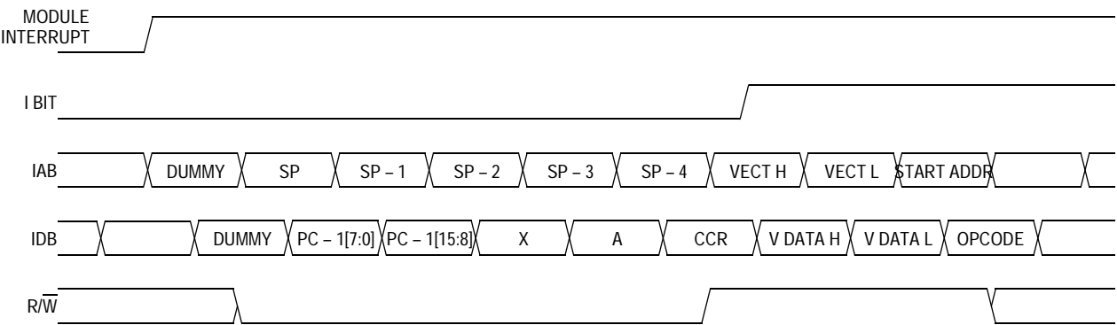
Figure 7-8. Interrupt Entry
