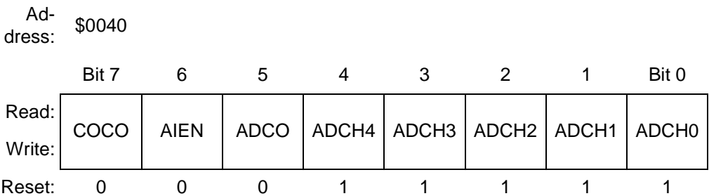
Figure 18-3. ADC Status and Control Register (ADSCR)
