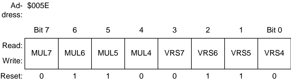
Figure 8-7. PLL Programming Register (PPG)
