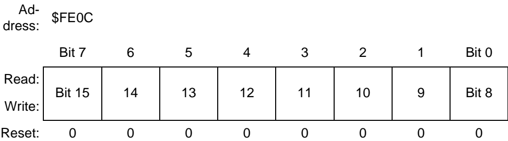
Figure 20-4. Break Address Register High (BRKH)
