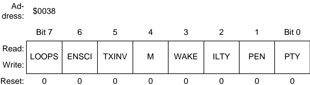
Figure 13-7. SCI Control Register 1 (SCC1)
