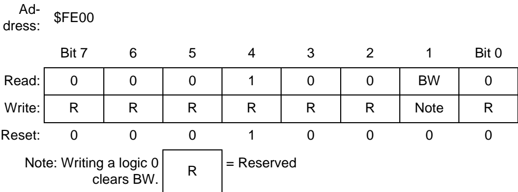
Figure 20-6. SIM Break Status Register (SBSR)
