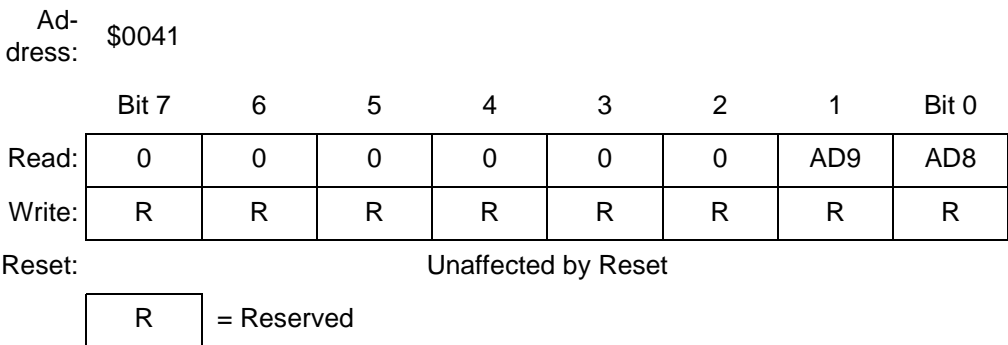
Figure 18-5. ADC Data Register High (ADRH) Right Justified Mode
