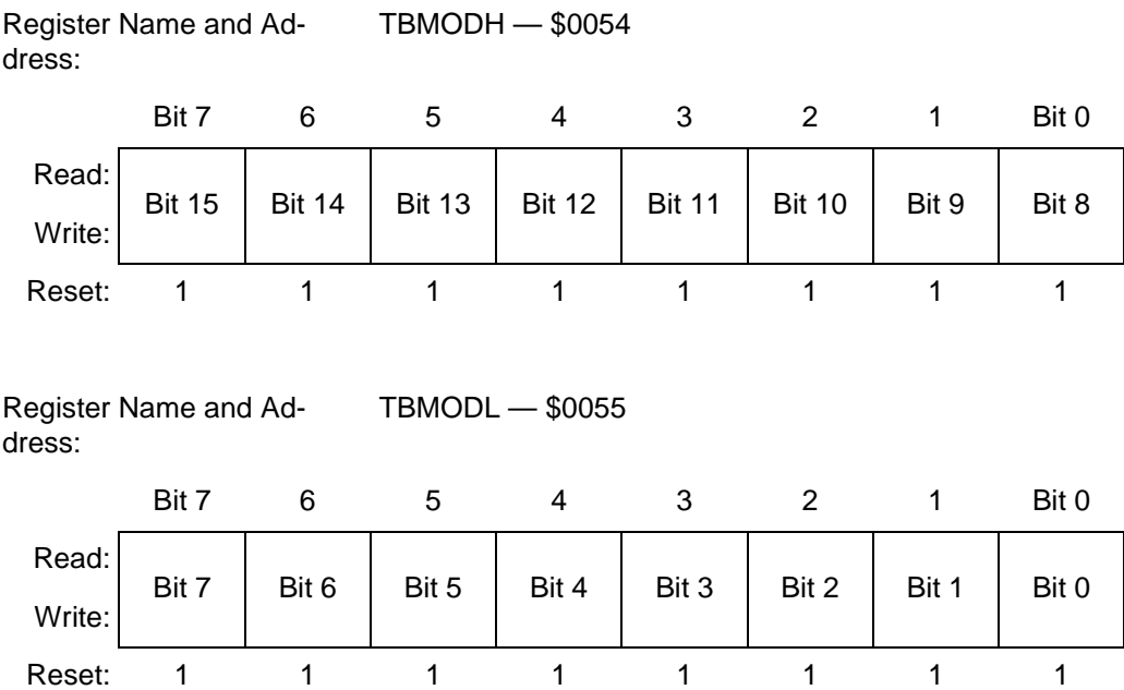
Figure 12-6. TIMB Counter Modulo Registers (TMODH and TMODL)
