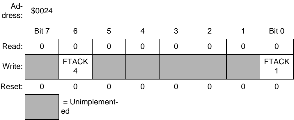
Figure 9-41. Fault Acknowledge Register (FTACK)
