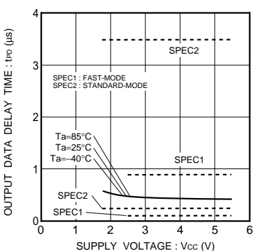
Fig.37 Output data delay time t_{po}
