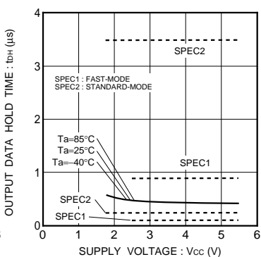
Fig.39 Output data hold time t_{po0}
