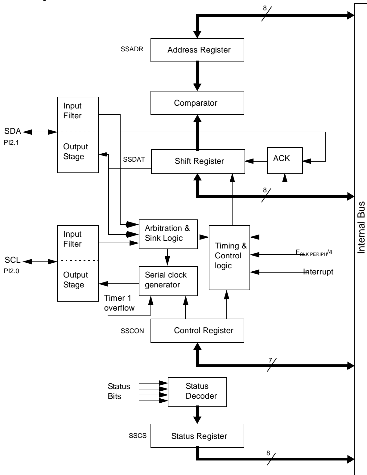
Figure 30. Block Diagram
