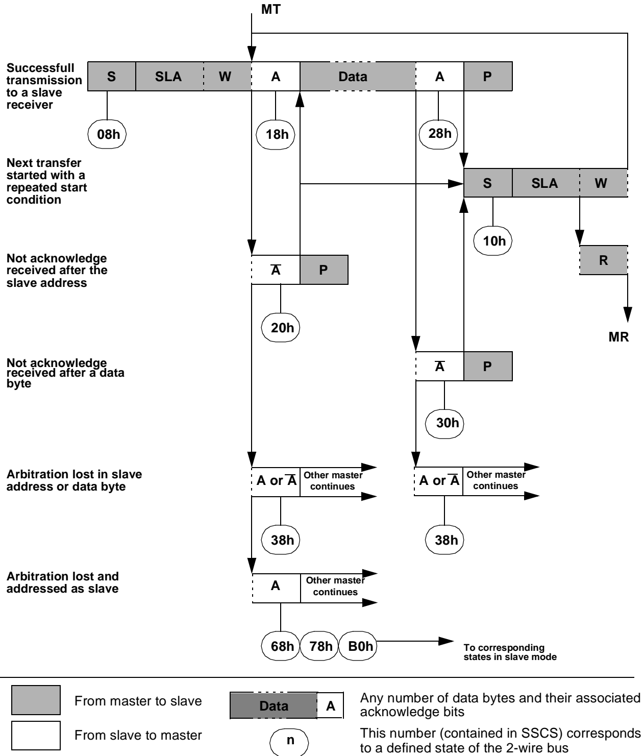
Figure 32. Format and State in the Master Transmitter Mode
