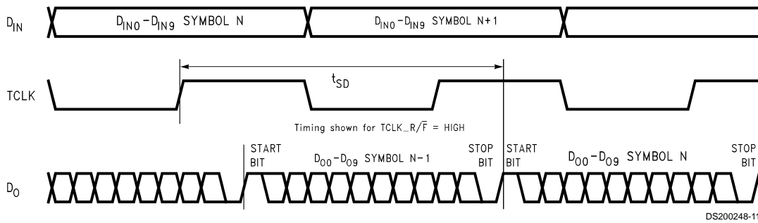
FIGURE 11. Serializer Delay
