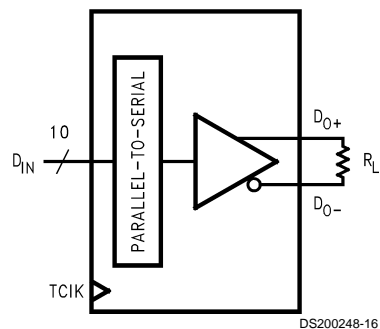
FIGURE 17. V_{OD} Diagram
