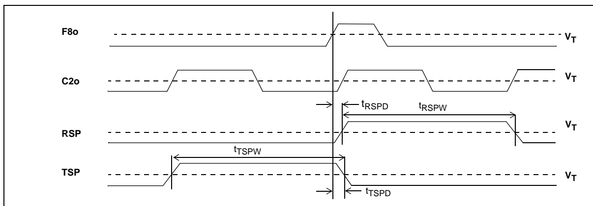
Figure 16 - Output Timing 2
