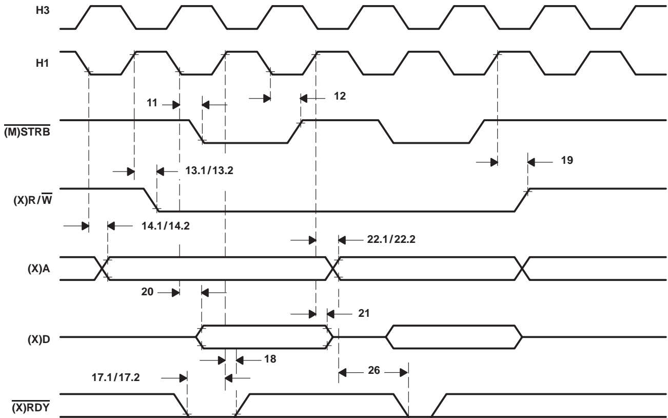
Figure 11. Timing for Memory [(\overline{M})\text{STRB} = 0] Write
