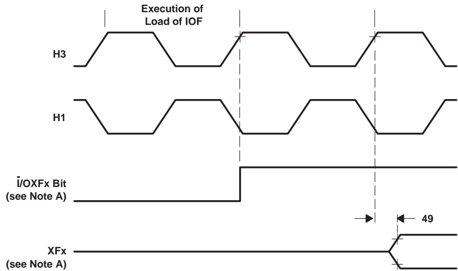
Figure 19. Timing for Change of XFx From Input to Output Mode
