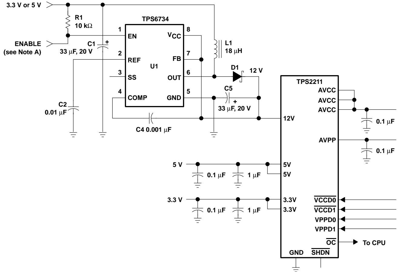
Figure 26. TPS2211 With TPS6734 12-V, 120-mA Supply
