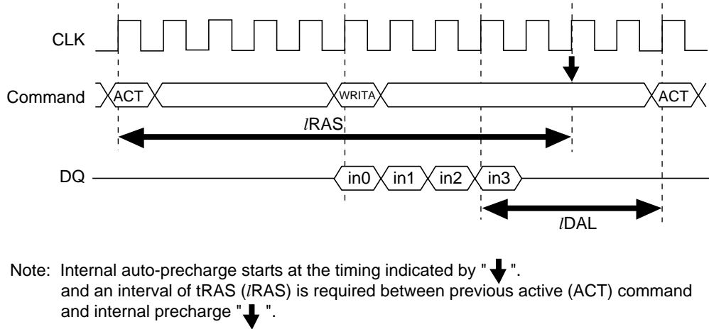
Burst Write (BL = 4)
