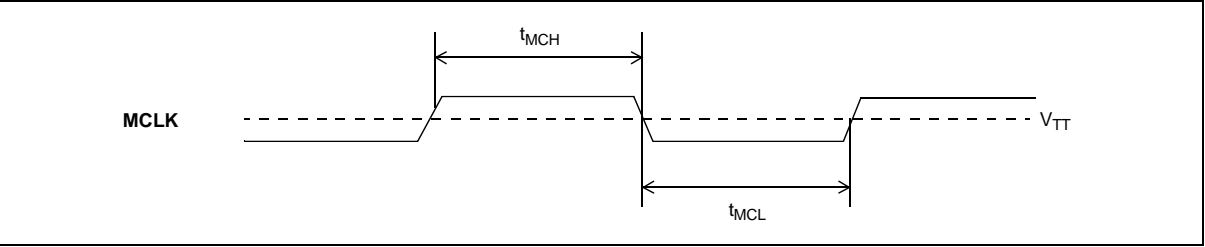
Figure 15 - Master Clock
