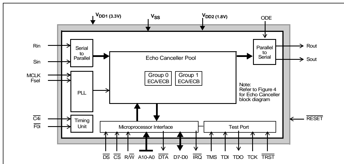
Figure 1 - ZL50233 Device Overview
