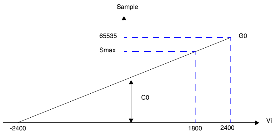
Figure 35. Gain Calculations
