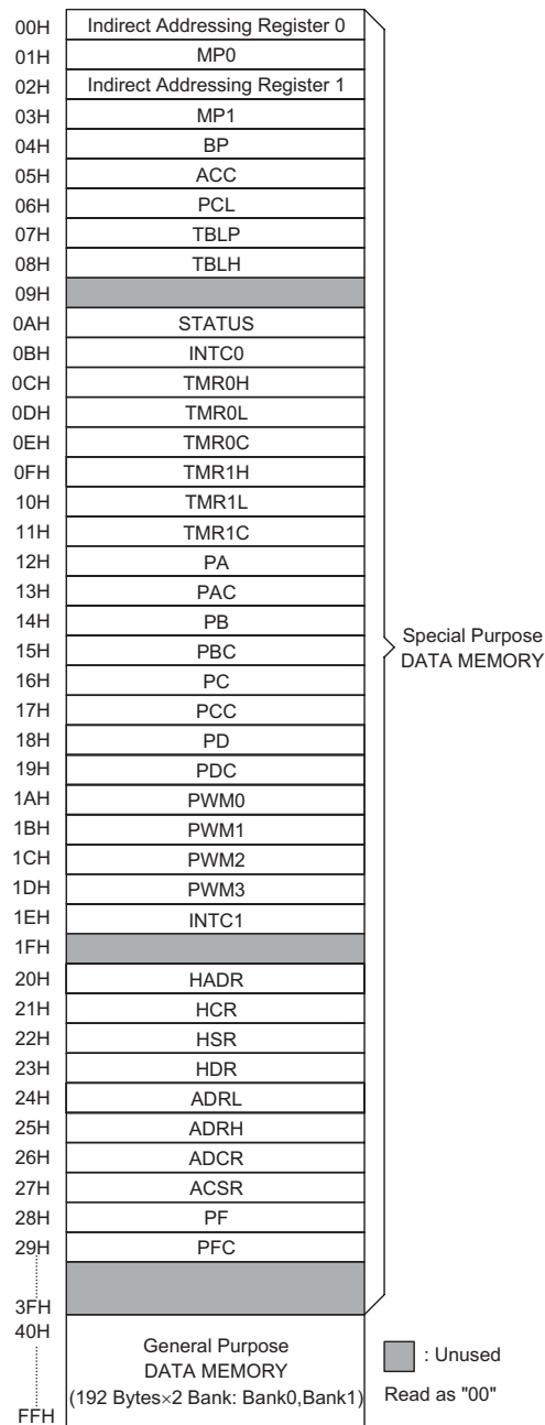
RAM Mapping
