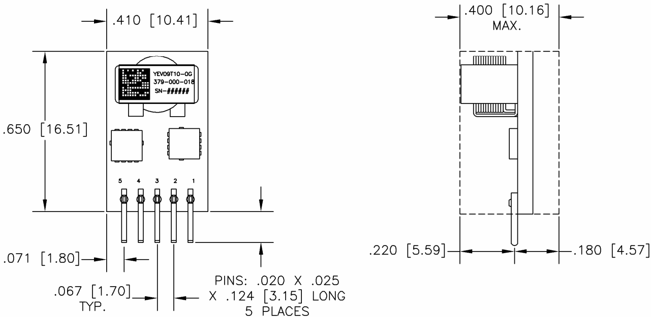
Figure 22. Mechanical Drawing
