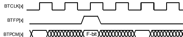
Figure 60: - Transmit Backplane: CMS=1, FE=0, DE=1, BTFP is Input
