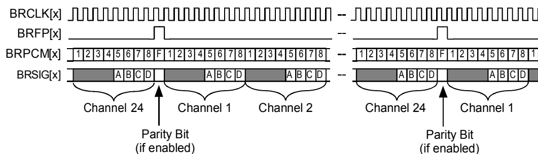
Figure 48: - T1 Receive Clock Slave: Full T1/E1 Mode
