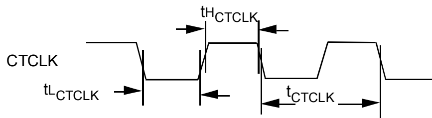
Figure 89: - Transmit Line Interface Timing
