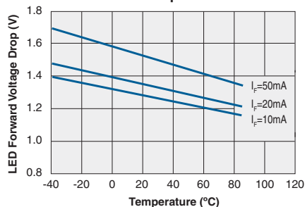
Typical Forward Voltage Drop vs. Temperature
