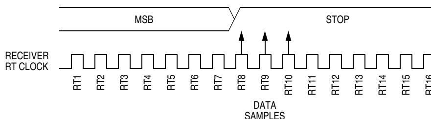
Figure 15-8. Slow Data
