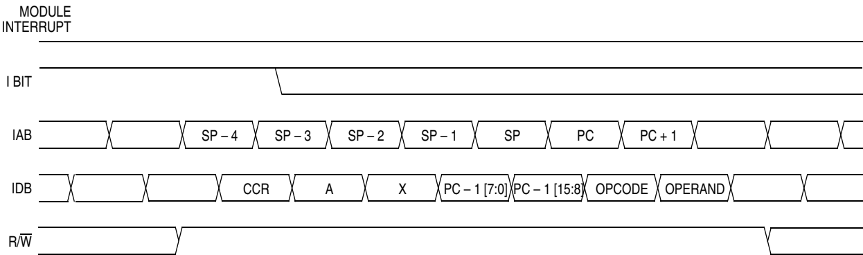
Figure 16-9. Interrupt Recovery Timing
