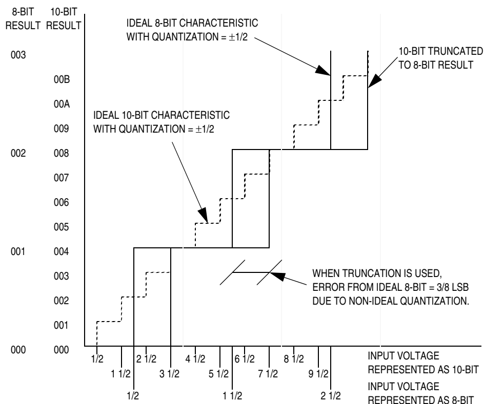
Figure 16-3. 8-Bit Truncation Mode Error
