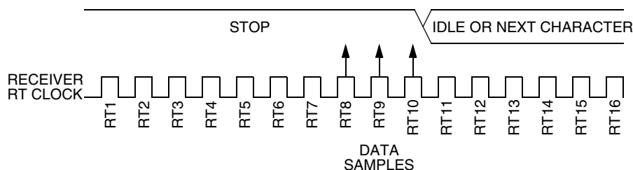
Figure 13-11. Fast Data
