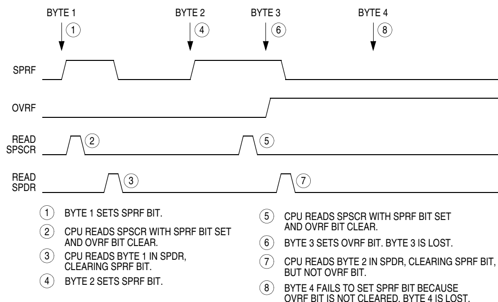
Figure 14-9. Missed Read of Overflow Condition
