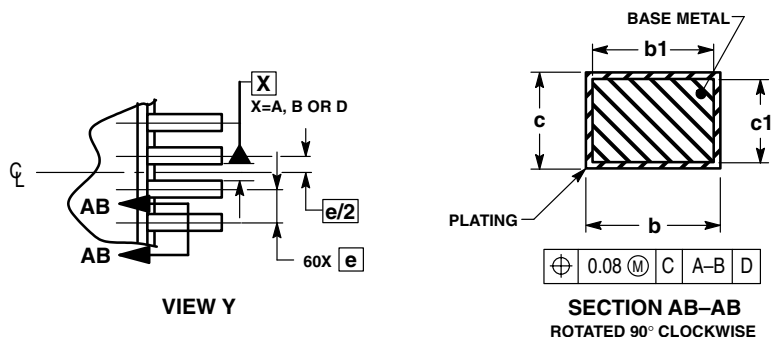
Figure 25-1. 64-Pin Low-Profile Quad Flat Pack (Case No. 840F)
