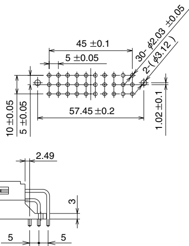
PCB mounting pattern
