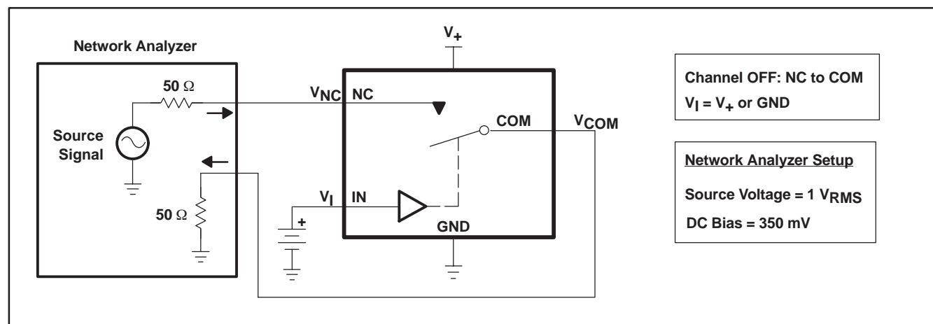
Figure 19. OFF Isolation ( O_{\text{ISO}} )
