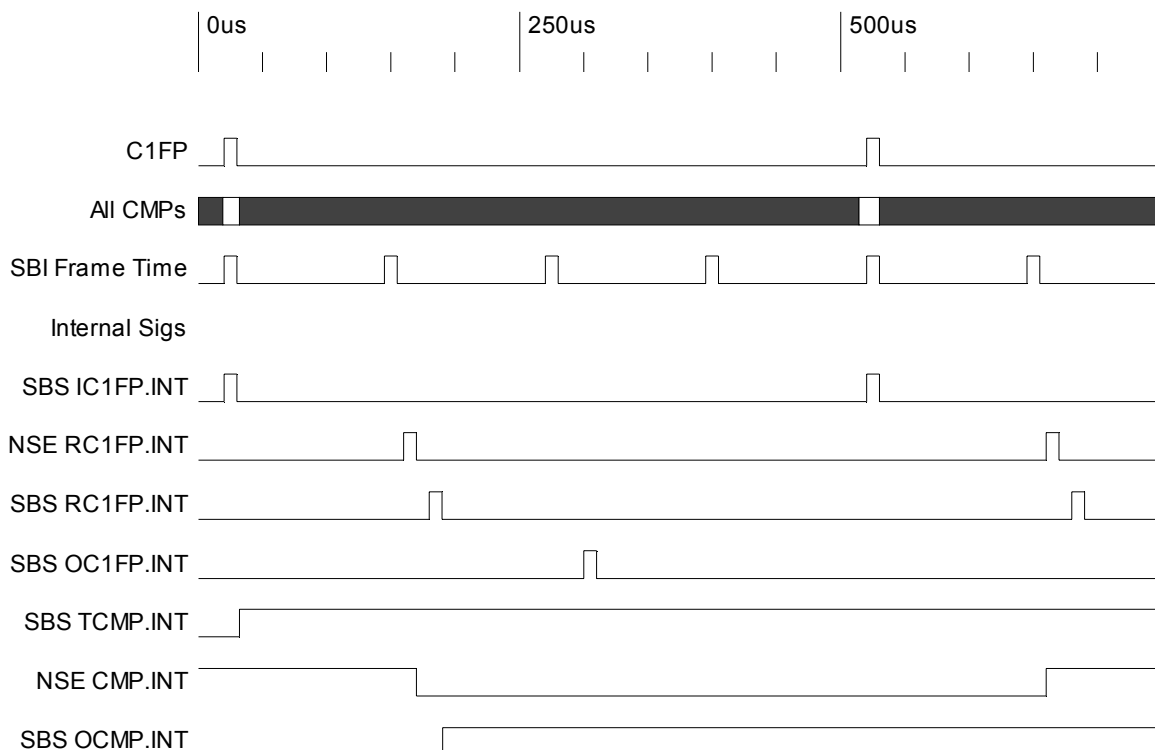
Figure 23 Switch Timing - DS0s without CAS
