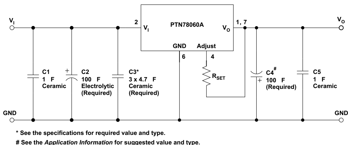
Figure 20. Adding High-Frequency Bypass Capacitors to the Input and Output
