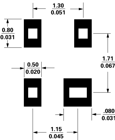
Figure 2. PCB Pad Layout for MSA-2743. Package dimensions in mm/inches.
