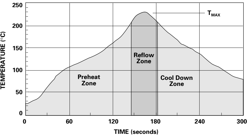
Figure 12. Surface Mount Assembly Profile.
