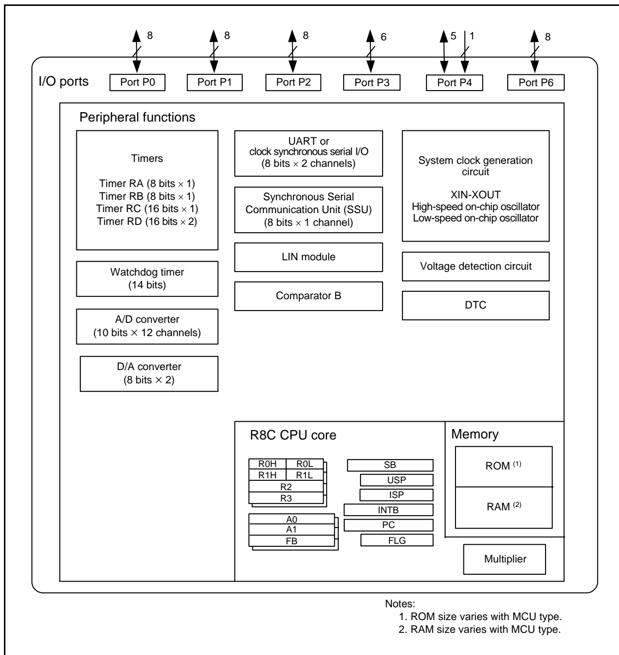
Figure 1.3 Block Diagram
