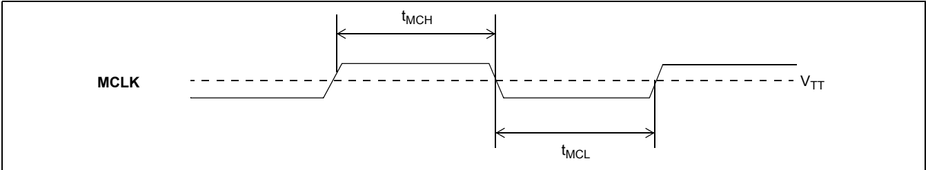
Figure 14 - Master Clock
