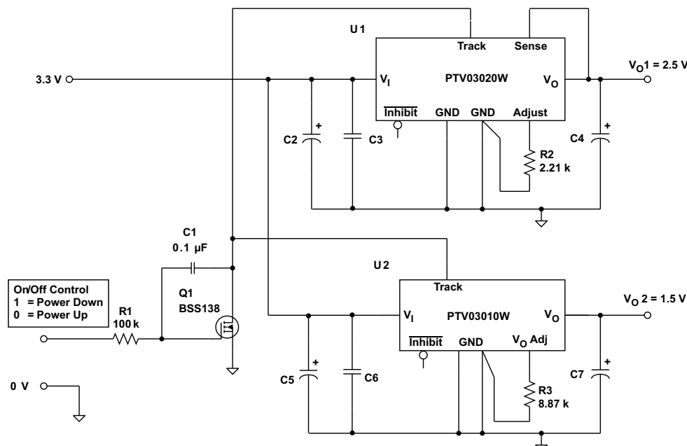
Figure 11. Sequenced Power Up and Power Down Using Auto-Track
