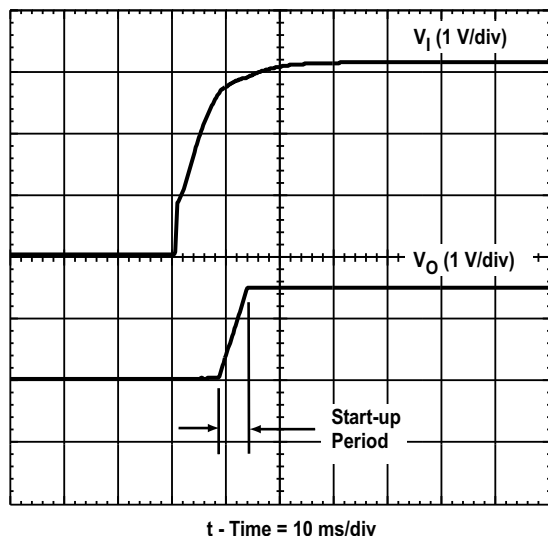
Figure 14. PTV03010W Start-Up
