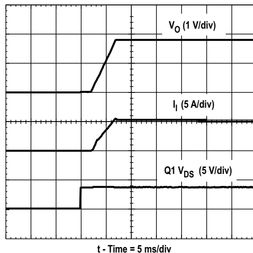
Figure 10. Inhibit Waveform
