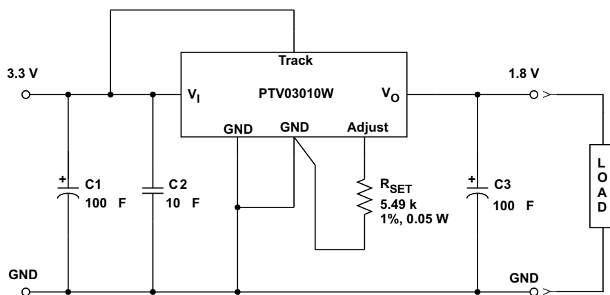
Figure 7. Power-Up Application Circuit
