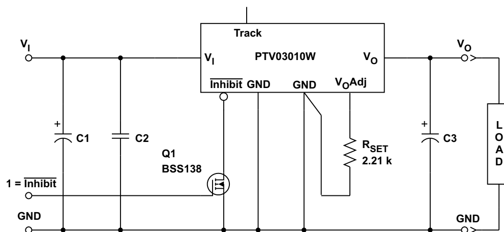
Figure 9. On/Off Inhibit Application Circuit
