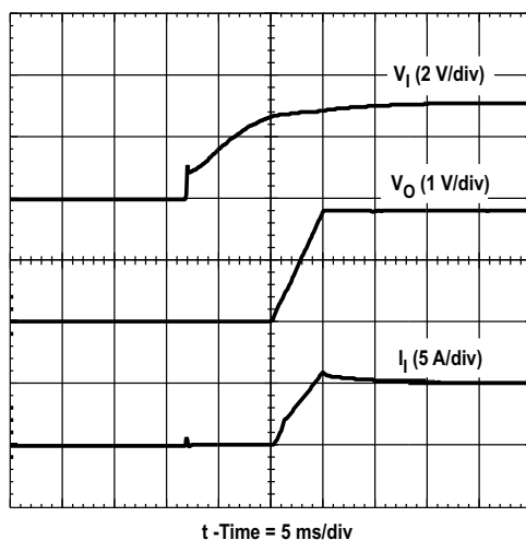
Figure 8. Power-Up Waveform
