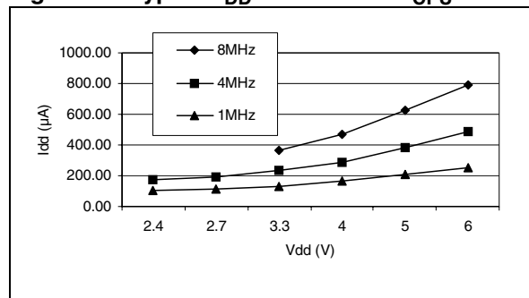
Figure 77. Typical I_{DD} in SLOW vs. f_{CPU}
