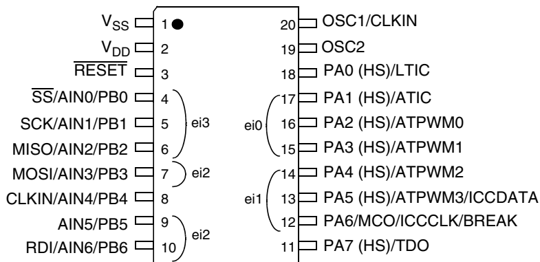
Figure 2. 20-Pin SO and DIP Package Pinout
