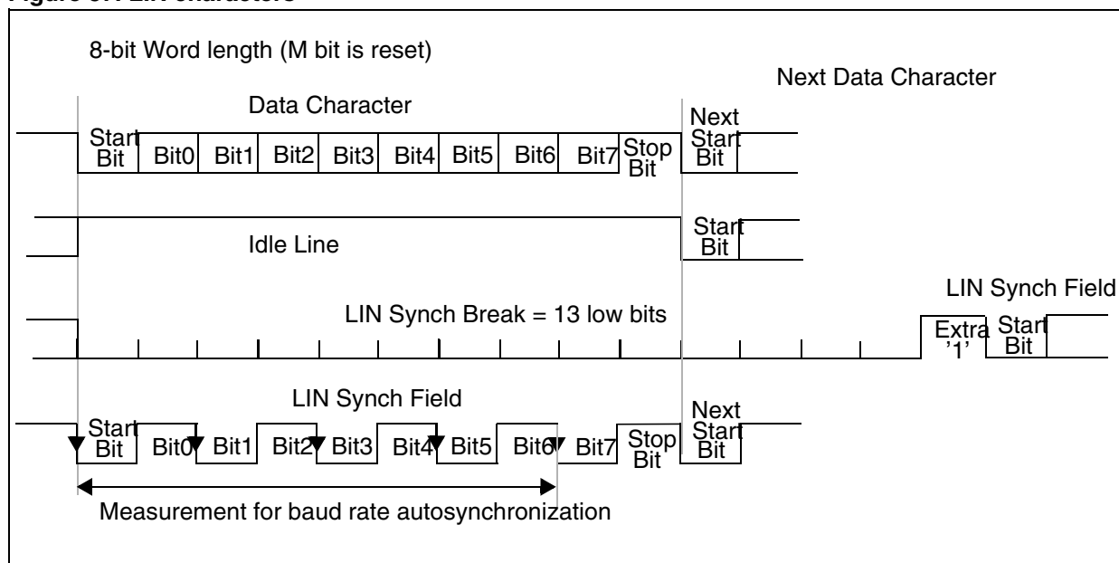
Figure 57. LIN characters
