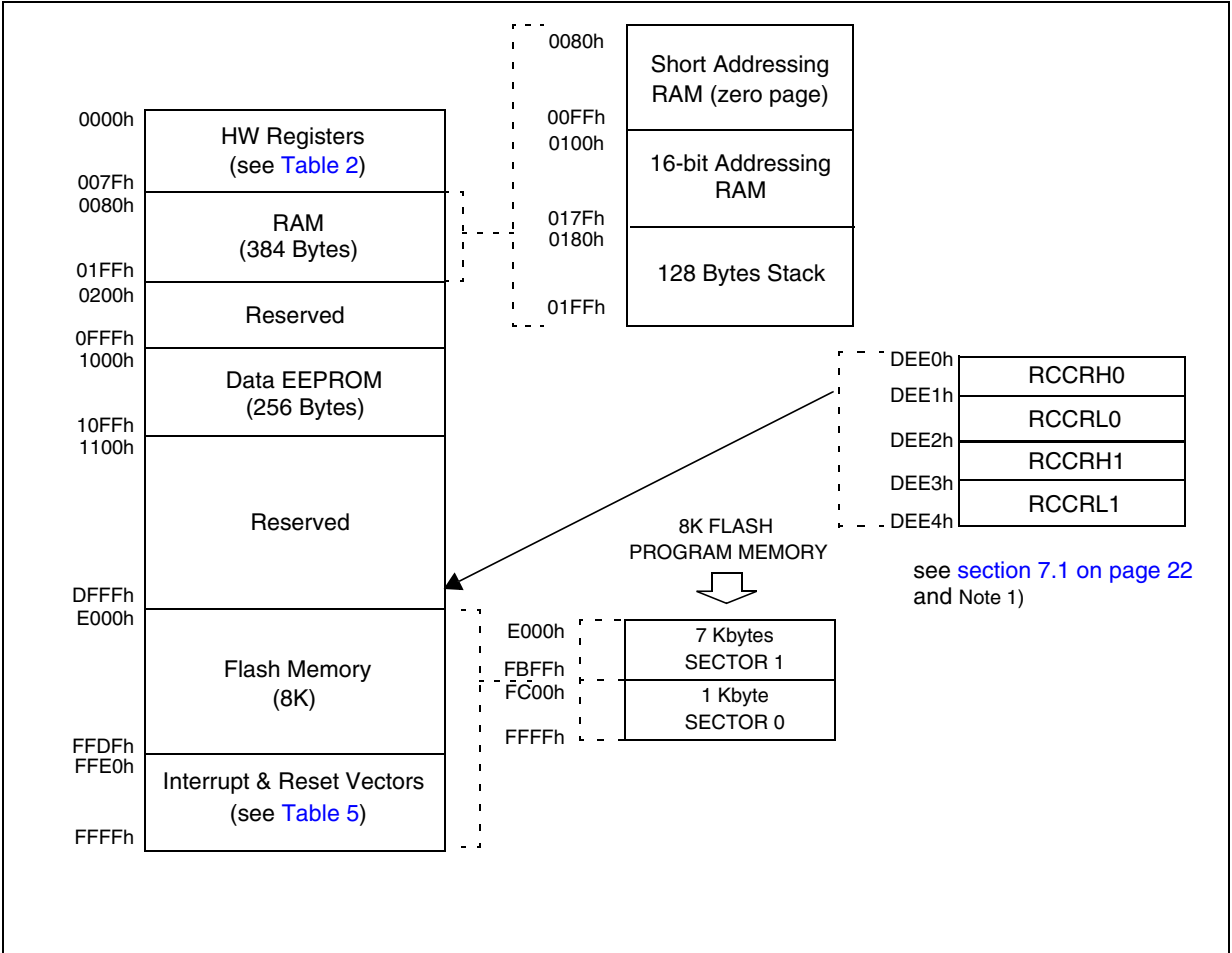
Figure 3. Memory Map
