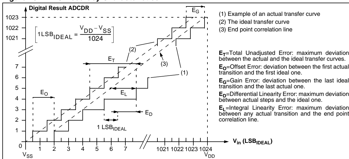
Figure 102. ADC Accuracy Characteristics
