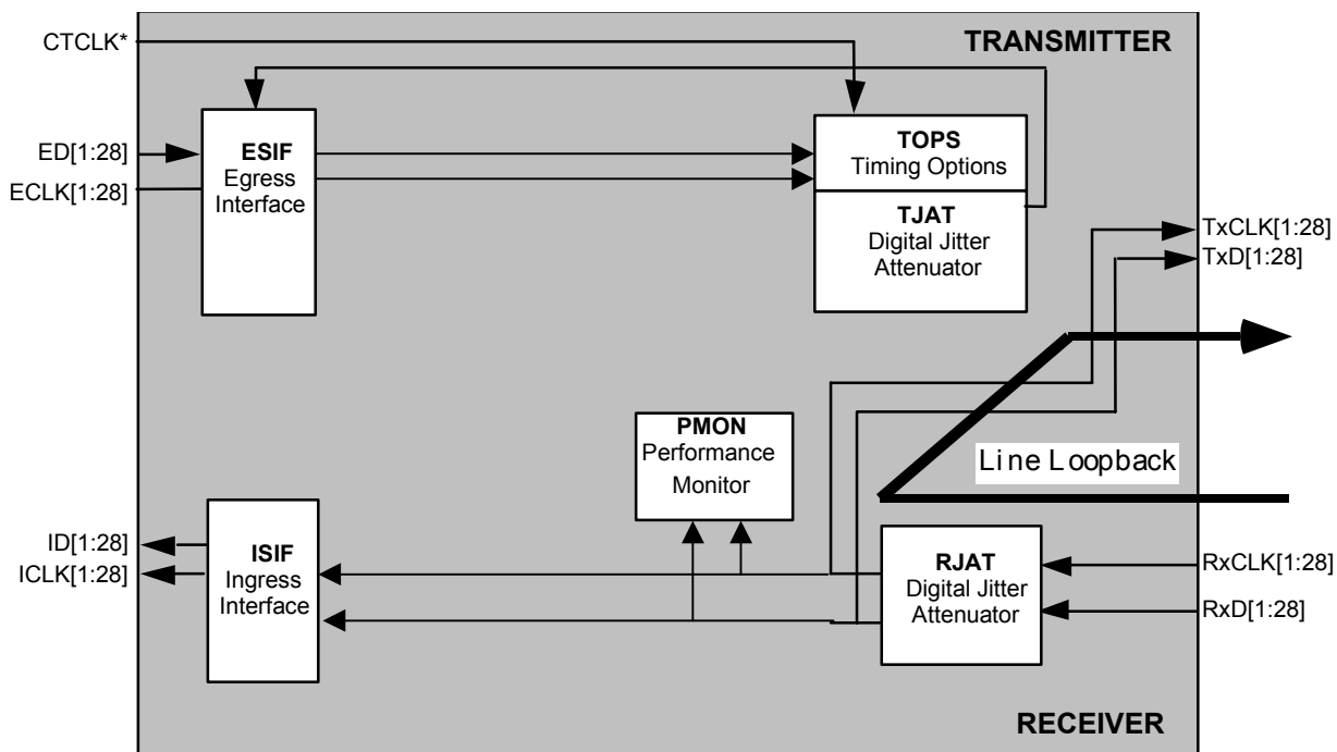
Figure 23: T1/E1 Line Loopback
