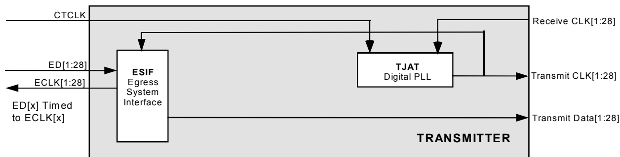
Figure 14 - Clock Master: Clear Channel
