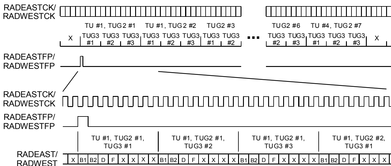
Figure 50: Remote Serial Alarm Port Timing
