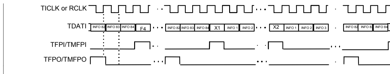
Figure 41: Framer Mode DS3 Transmit Input Stream
