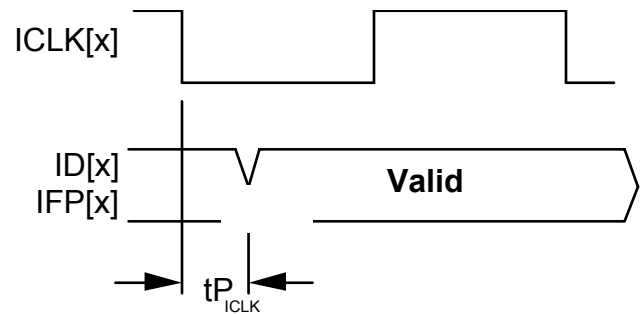
Figure 68: Ingress Interface Timing - Clock Master Modes
