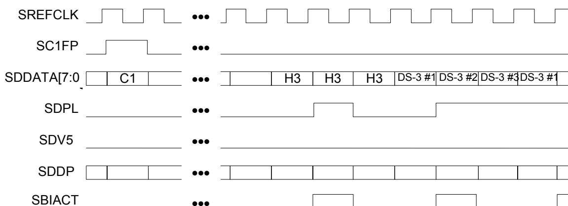
Figure 52: SBI DROP Bus DS3 Functional Timing
