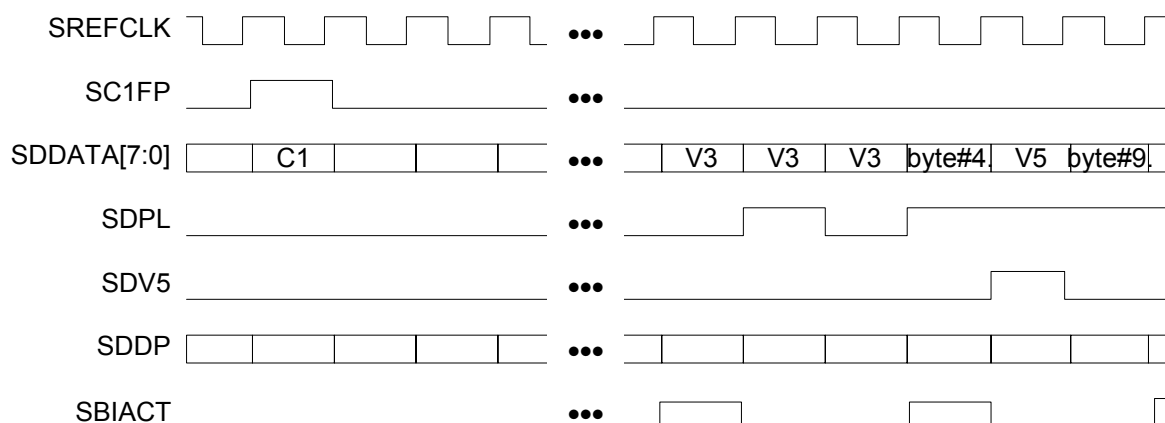
Figure 51: SBI DROP Bus T1/E1 Functional Timing
