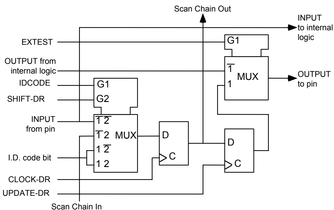
Figure 35: Bidirectional Cell (IO_CELL)
