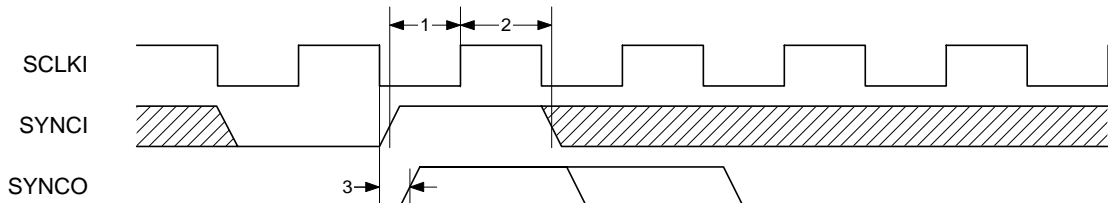
Figure 22 Timing of SYNCI and SYNCO
