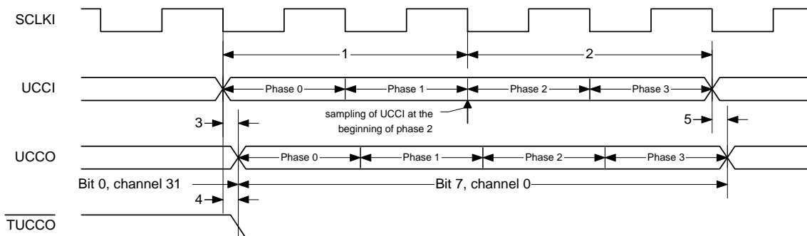
Figure 26 Special Cases for Multiframe Alignment and Timing Characteristics
