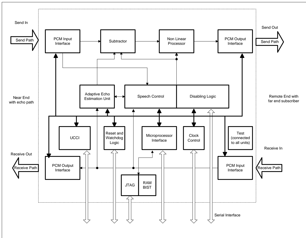
Figure 7 Block Diagram
