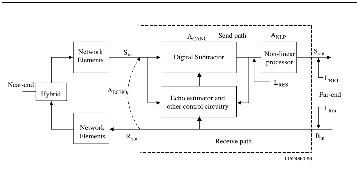
Figure 42 Location of levels and loss of an echo canceller
