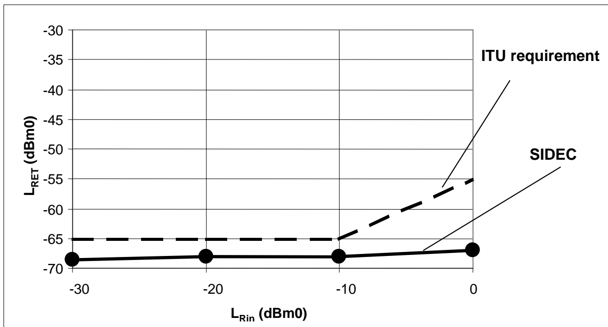
Figure 39 SIDEC steady state behavior with NLP enabled
