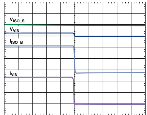
Figure 26. VBUS Disconnect
