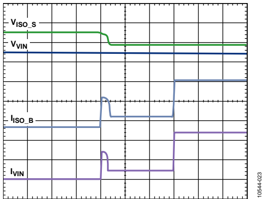
Figure 23. Charging Startup, V_{IN} = 5.0\text{ V} , ILIM[3:0] = 0110 (Binary) = 500 mA, ICHG[4:0] = 01110 (Binary) = 750 mA
