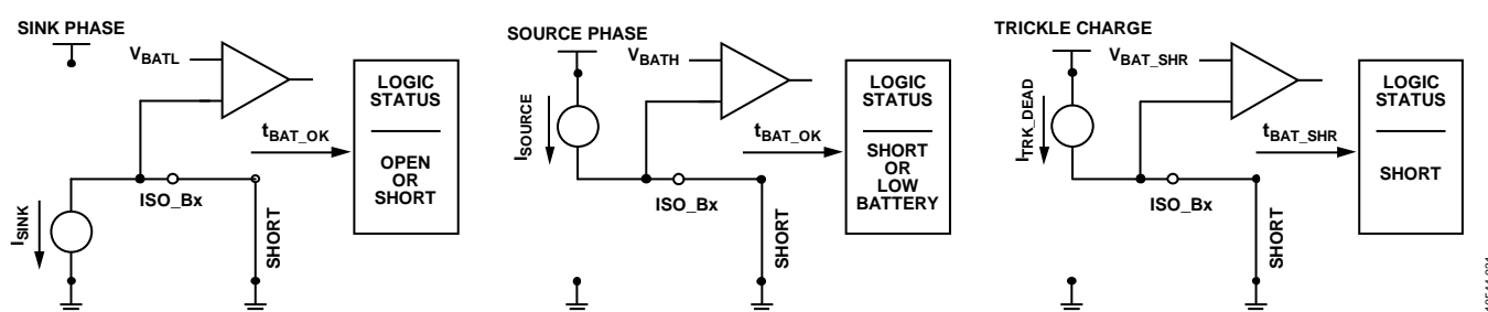
Figure 31. Trickle Charge
