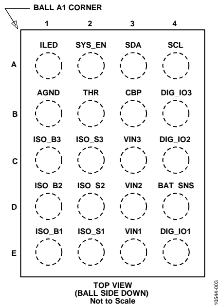
Figure 3. Pin Configuration
