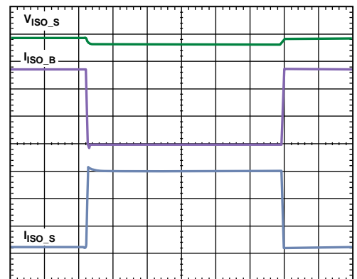
Figure 27. Load Transient, I_{ISO\_SX} Load = 300 mA to 1500 mA to 300 mA, EN\_CHG = \text{High} , ILIM[3:0] = 0110 (Binary) = 500 mA
