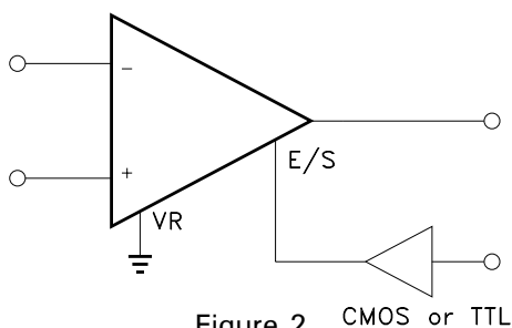
Figure 2 CMOS or TTL Output Disable with a Single Supply
