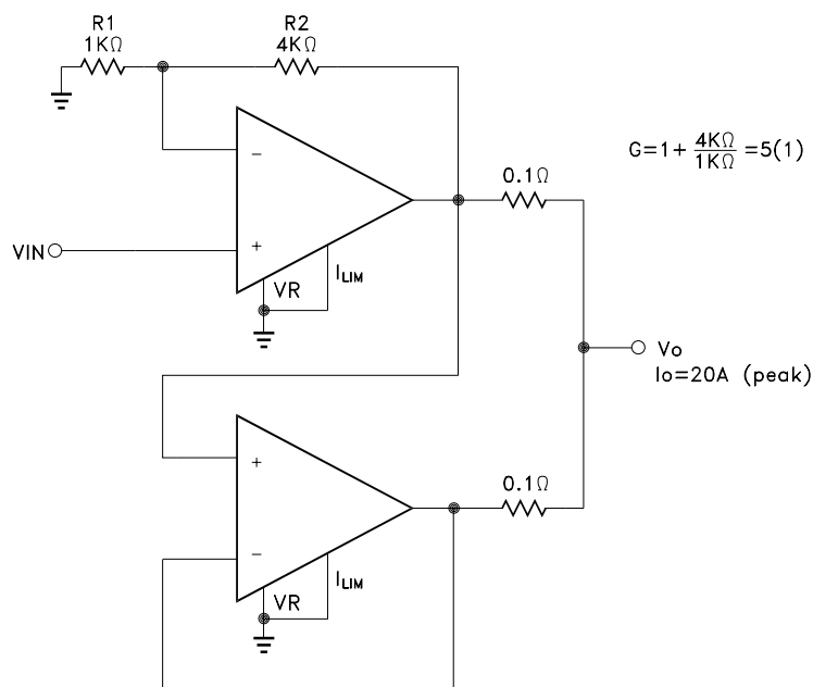
Figure 5 Parallel Output For Increased Output Current
