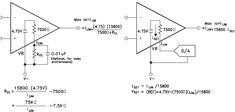
Figure 1 Adjustable Current Limit
