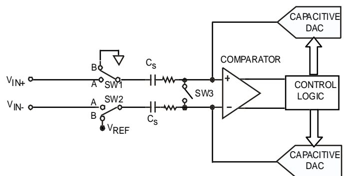
Figure 4. ADC Conversion Phase
