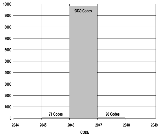
TPC 15. Histogram of 10000 conversions of a DC Input with V_{DD} = 3V
